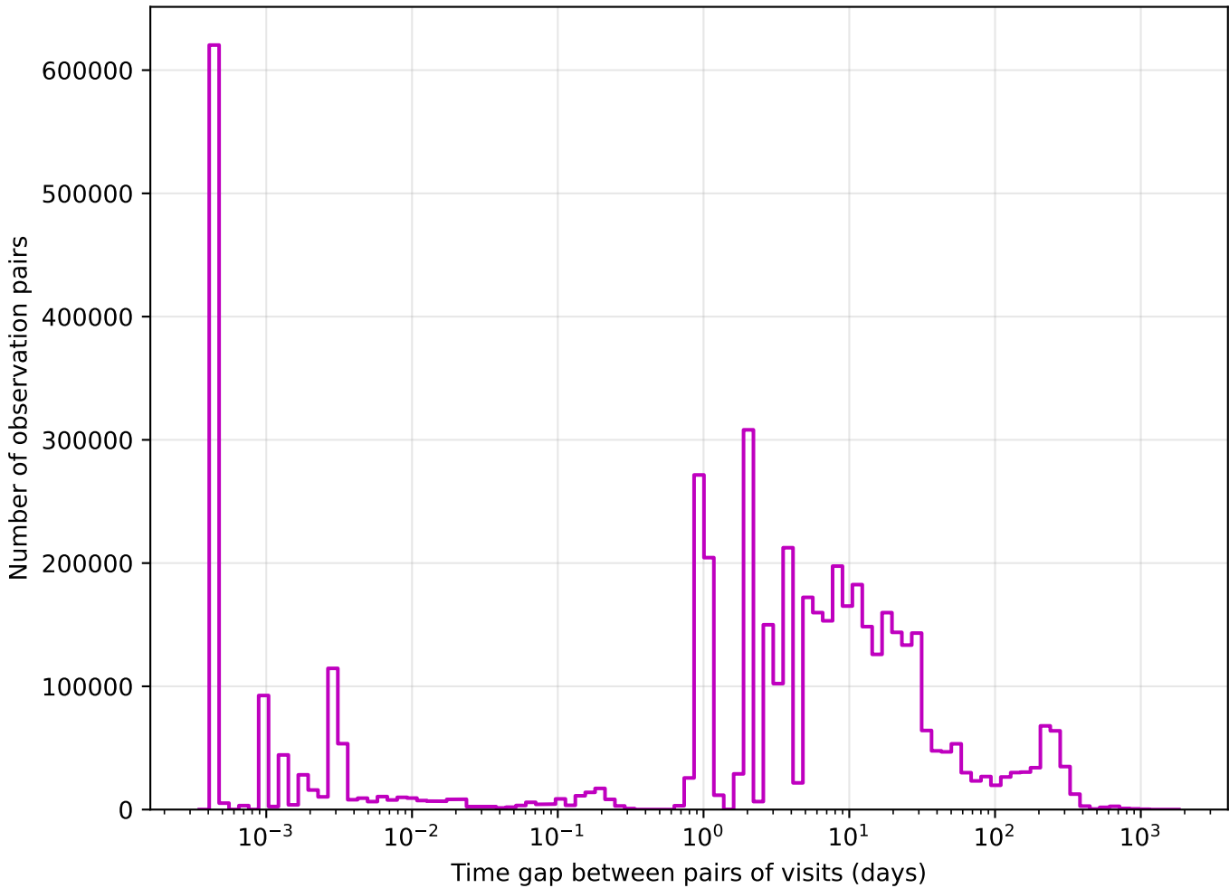
weather_cloudso18v3.4_10yrs z band: Tgaps observationStartMJD
