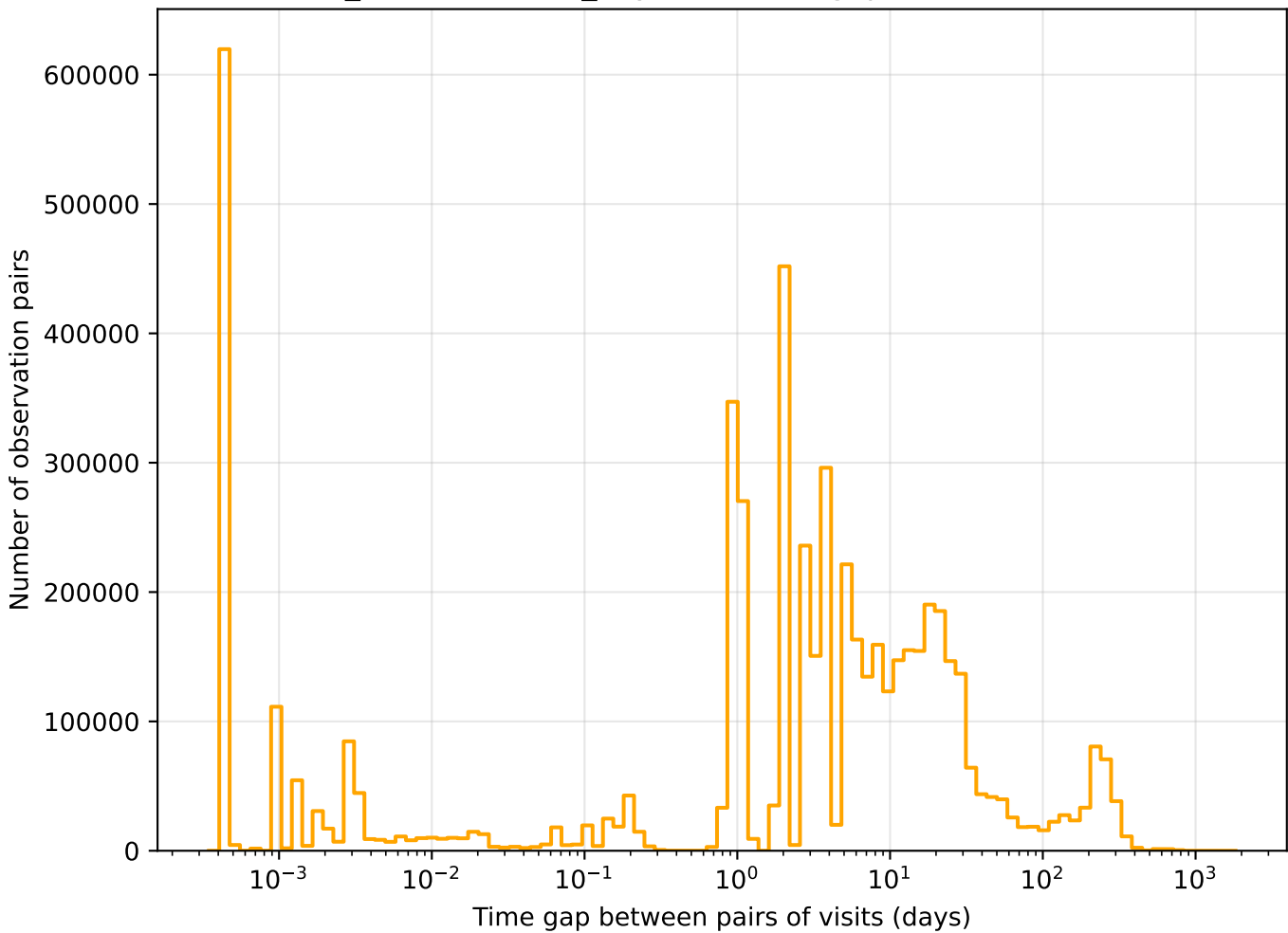
weather_cloudso18v3.4_10yrs r band: Tgaps observationStartMJD
