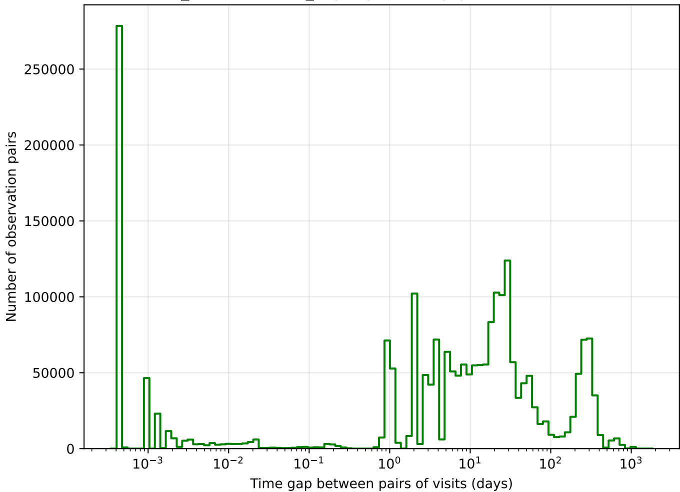
weather_cloudso18v3.4_10yrs g band: Tgaps observationStartMJD
