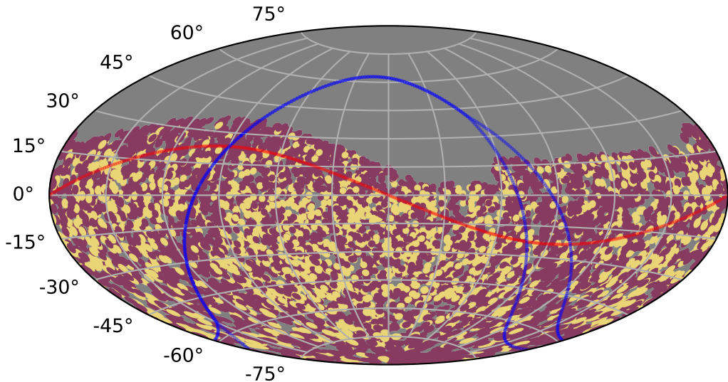
weather_cloudso18v3.4_10yrs : TDEsPopMetric_prepeak
