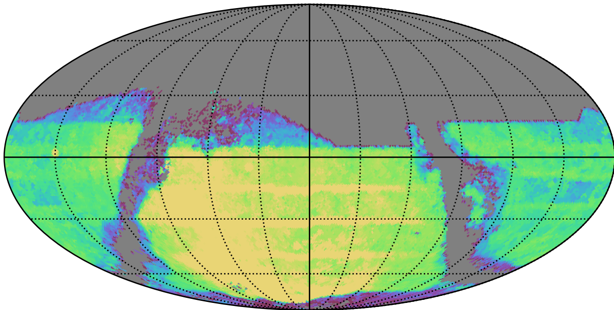
weather_cloudso18v3.4_10yrs : TDC_season
