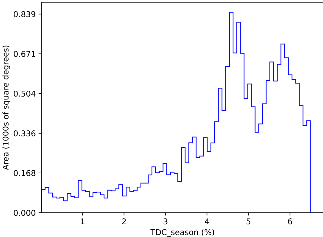
weather_cloudso18v3.4_10yrs : TDC_season
