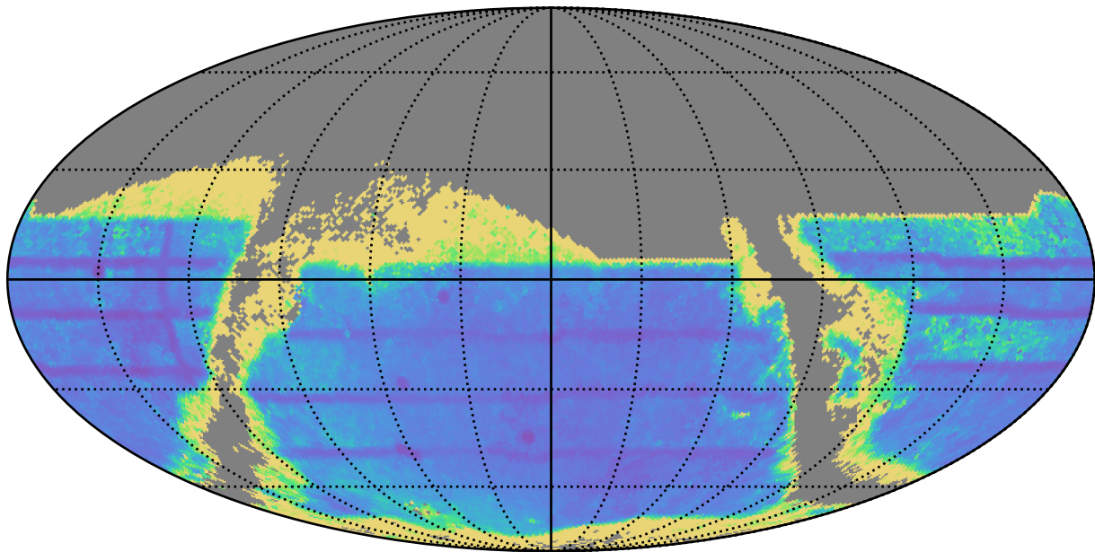
weather_cloudso18v3.4_10yrs : TDC_precision
