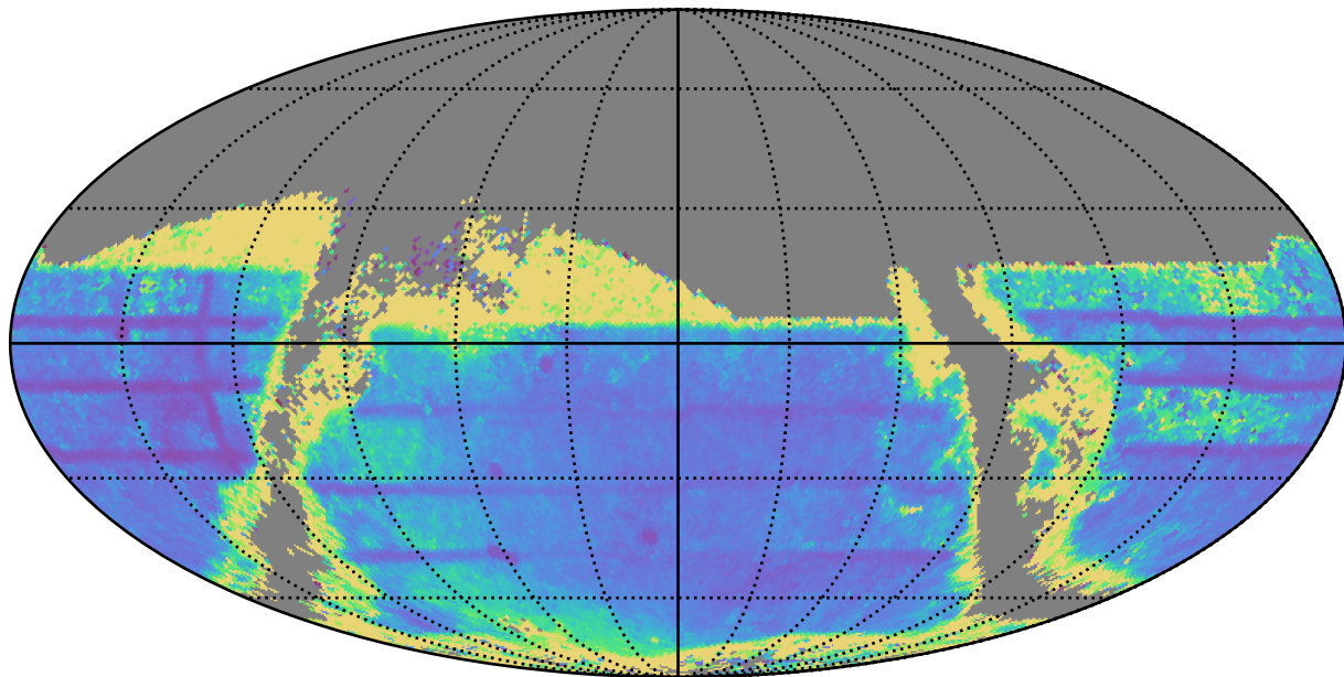
weather_cloudso18v3.4_10yrs : TDC_cadence
