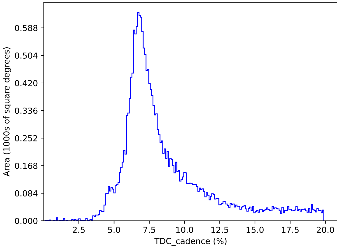
weather_cloudso18v3.4_10yrs : TDC_cadence
