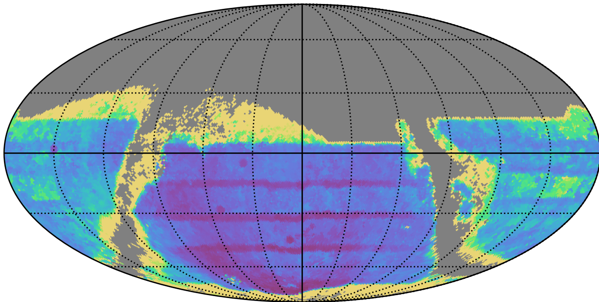
weather_cloudso18v3.4_10yrs : TDC_accuracy
