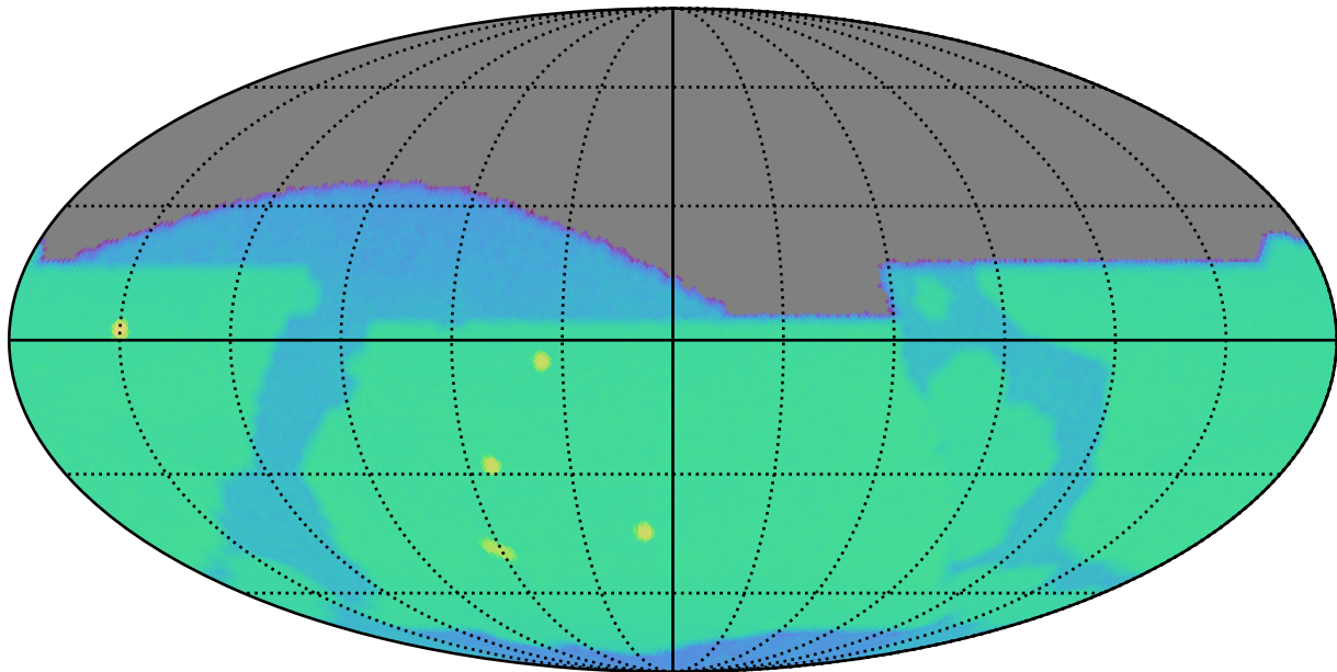
weather_cloudso18v3.4_10yrs z: SurfaceBrightLimit
