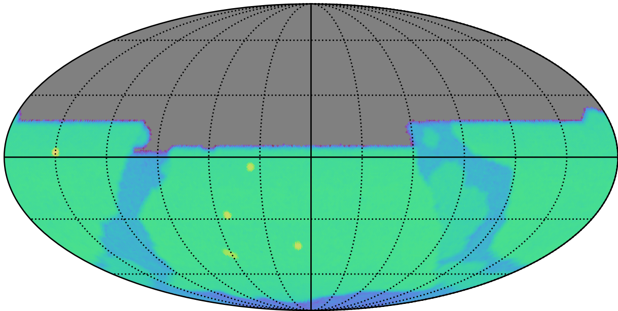
weather_cloudso18v3.4_10yrs y: SurfaceBrightLimit
