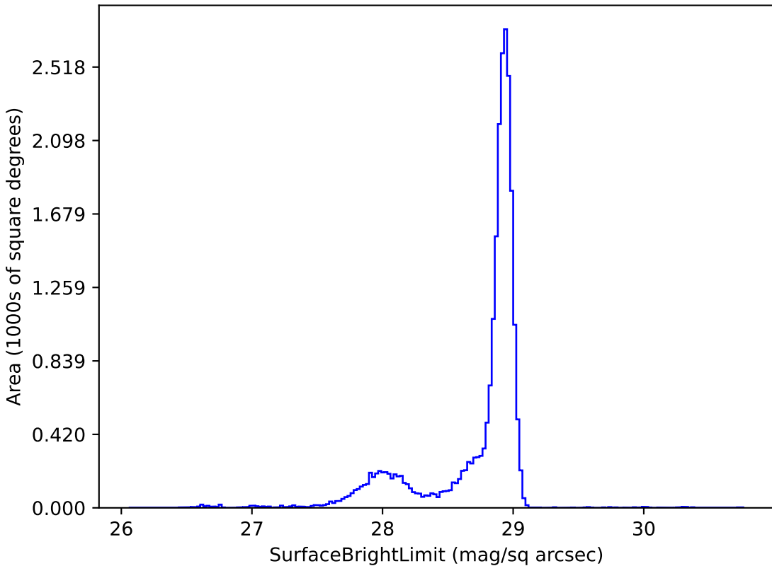
weather_cloudso18v3.4_10yrs u: SurfaceBrightLimit
