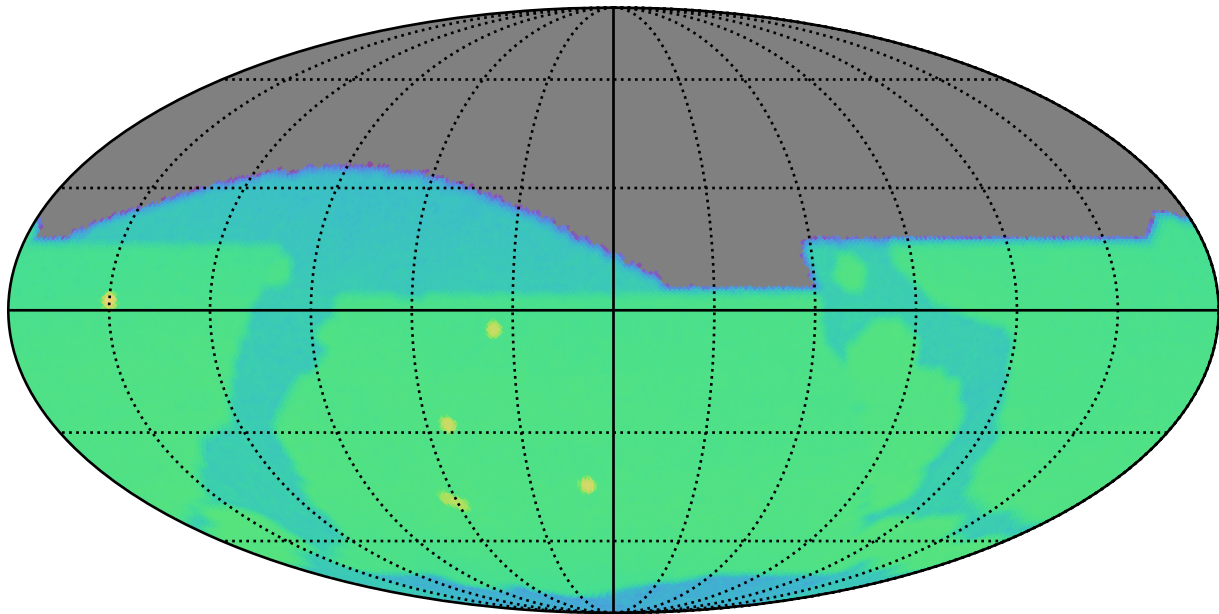
weather_cloudso18v3.4_10yrs r: SurfaceBrightLimit
