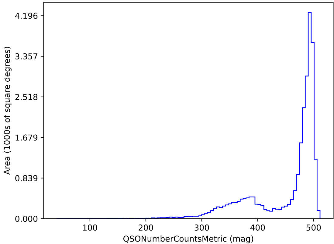
weather_cloudso18v3.4_10yrs z band and non-DD: QSONumberCountsMetric
