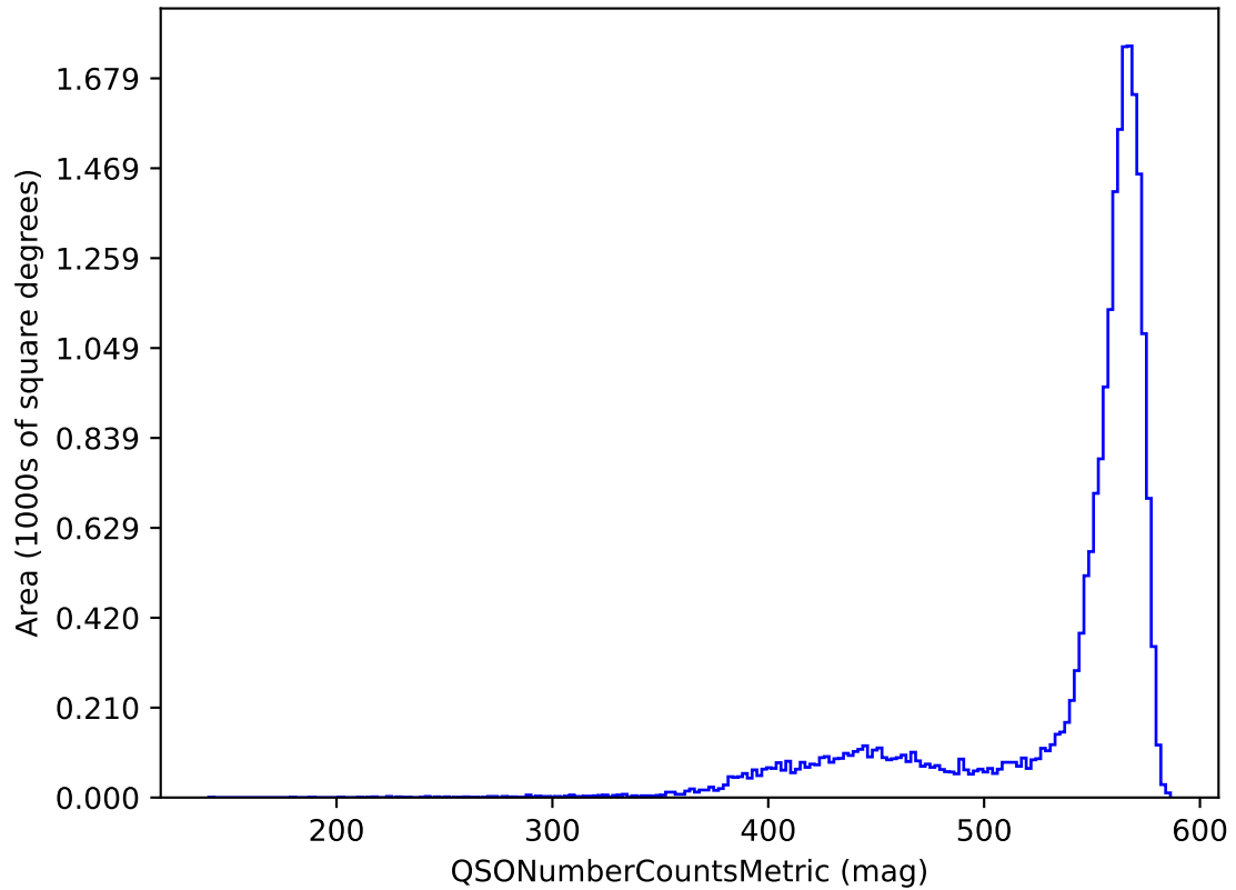
weather_cloudso18v3.4_10yrs y band and non-DD: QSONumberCountsMetric
