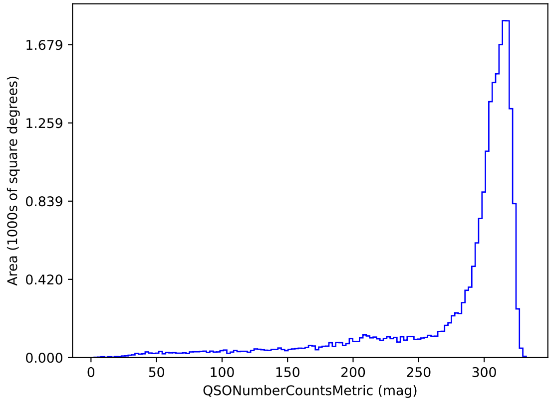
weather_cloudso18v3.4_10yrs u band and non-DD: QSONumberCountsMetric
