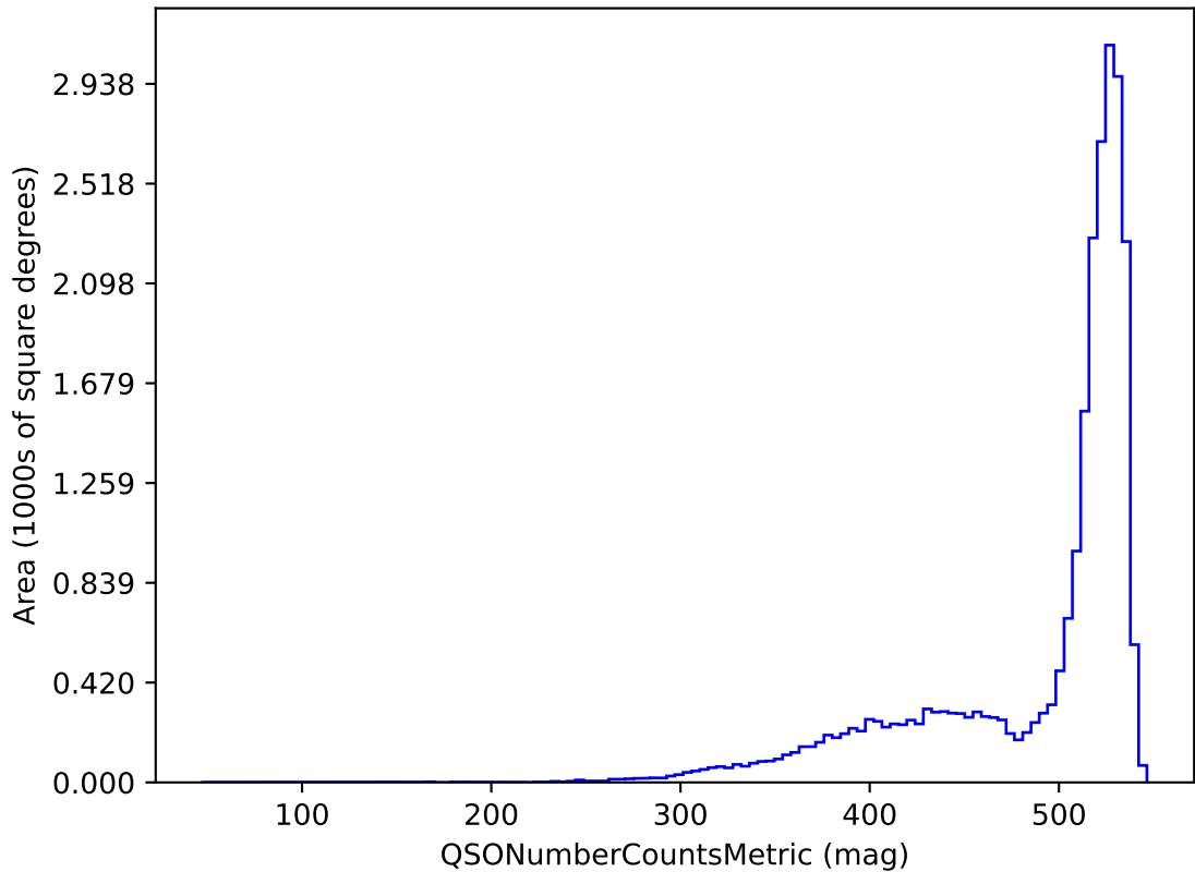
weather_cloudso18v3.4_10yrs r band and non-DD: QSONumberCountsMetric
