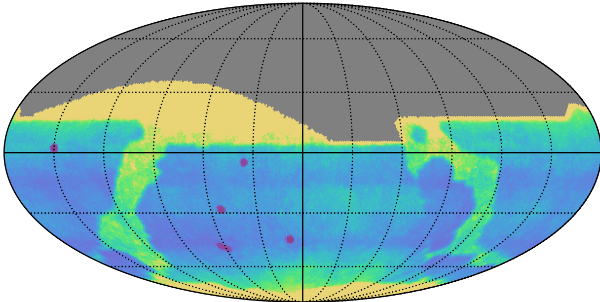
weather_cloudso18v3.4_10yrs : Proper Motion Uncert @ 24.0
