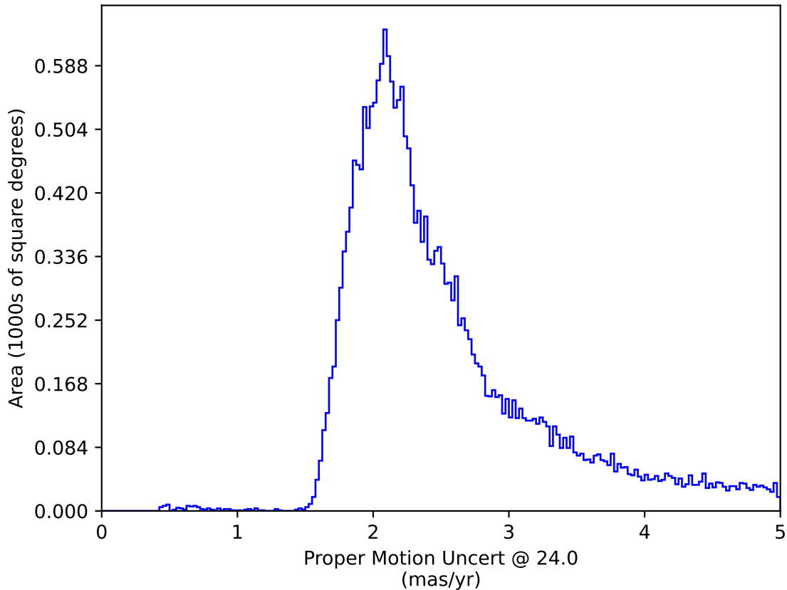
weather_cloudso18v3.4_10yrs : Proper Motion Uncert @ 24.0
