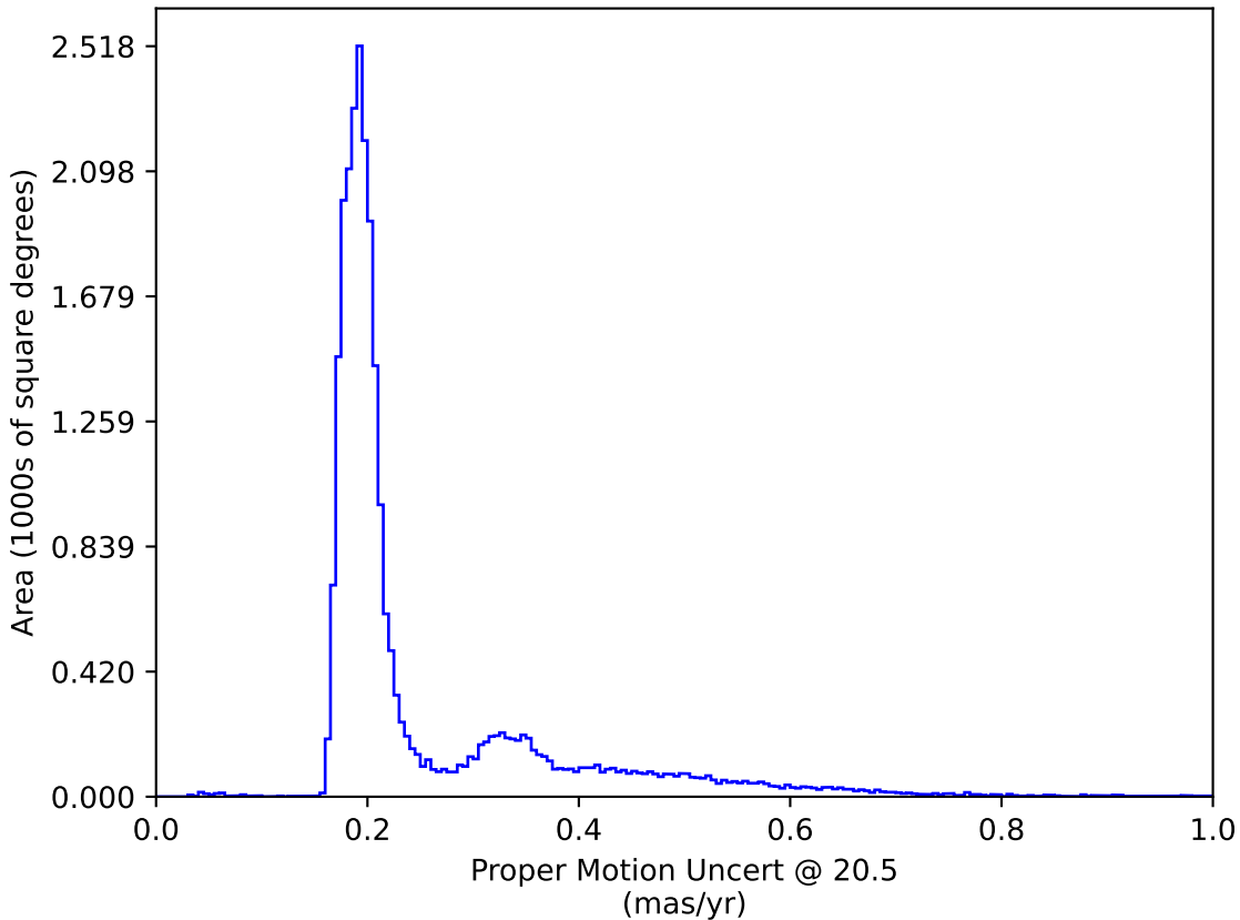
weather_cloudso18v3.4_10yrs : Proper Motion Uncert @ 20.5
