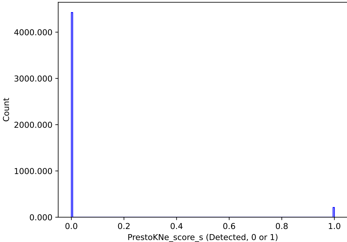
weather_cloudso18v3.4_10yrs : PrestoKNe_score_s
