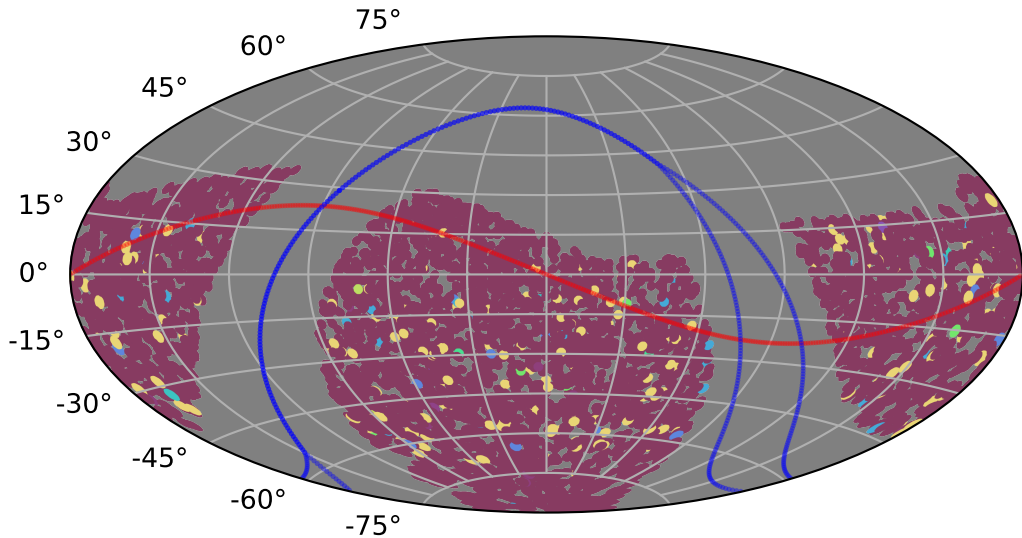
weather_cloudso18v3.4_10yrs : PrestoKNe_score_p
