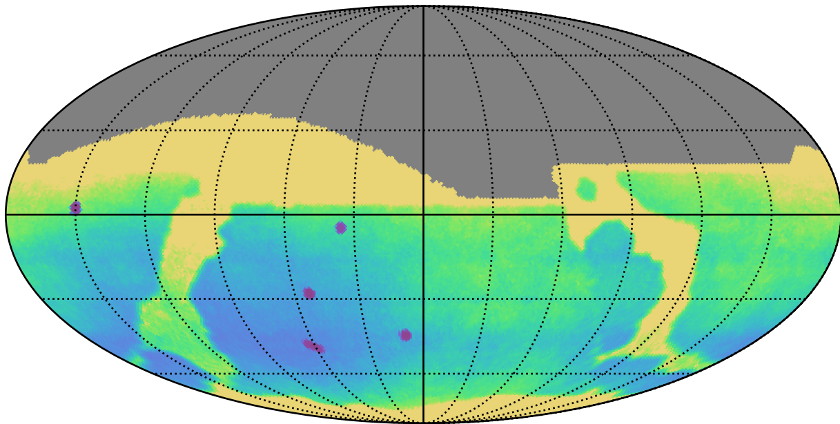
weather_cloudso18v3.4_10yrs : Parallax Uncert @ 24.0
