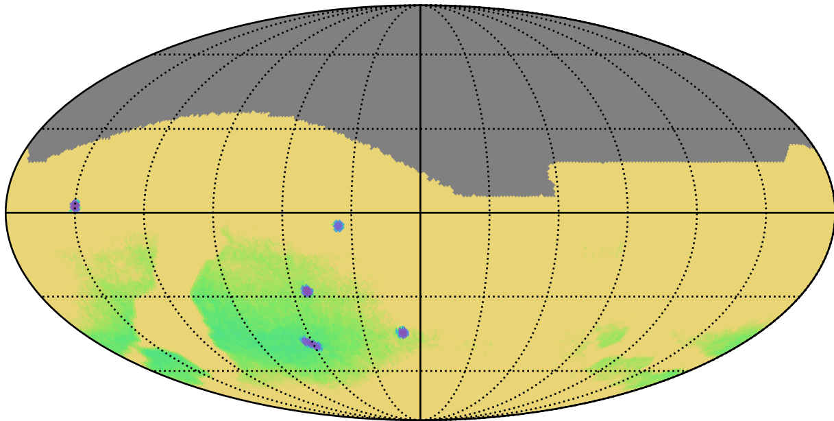
weather_cloudso18v3.4_10yrs : Parallax Uncert @ 22.4
