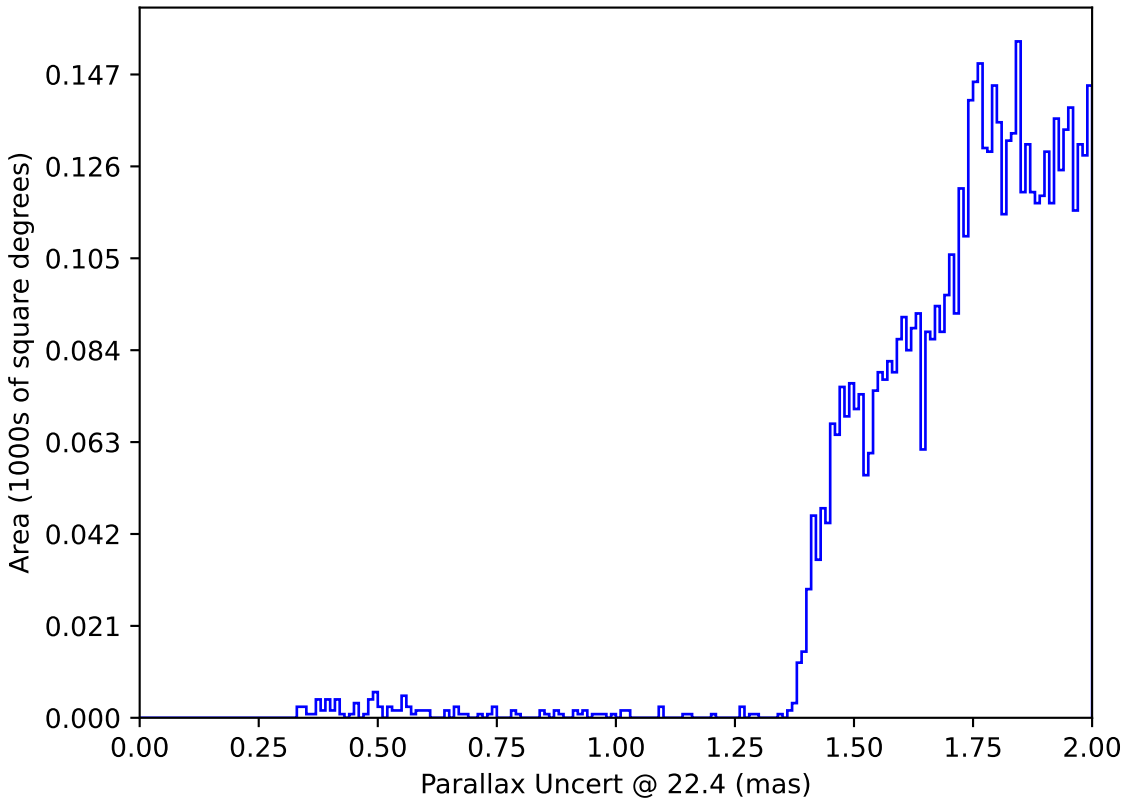
weather_cloudso18v3.4_10yrs : Parallax Uncert @ 22.4
