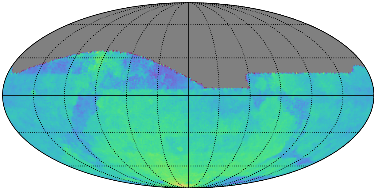
weather_cloudso18v3.4_10yrs : Parallax Coverage @ 24.0
