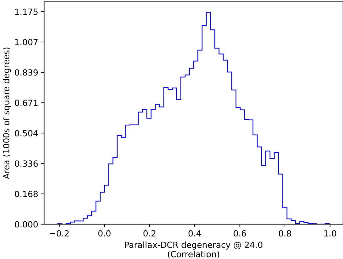
weather_cloudso18v3.4_10yrs : Parallax-DCR degeneracy @ 24.0
