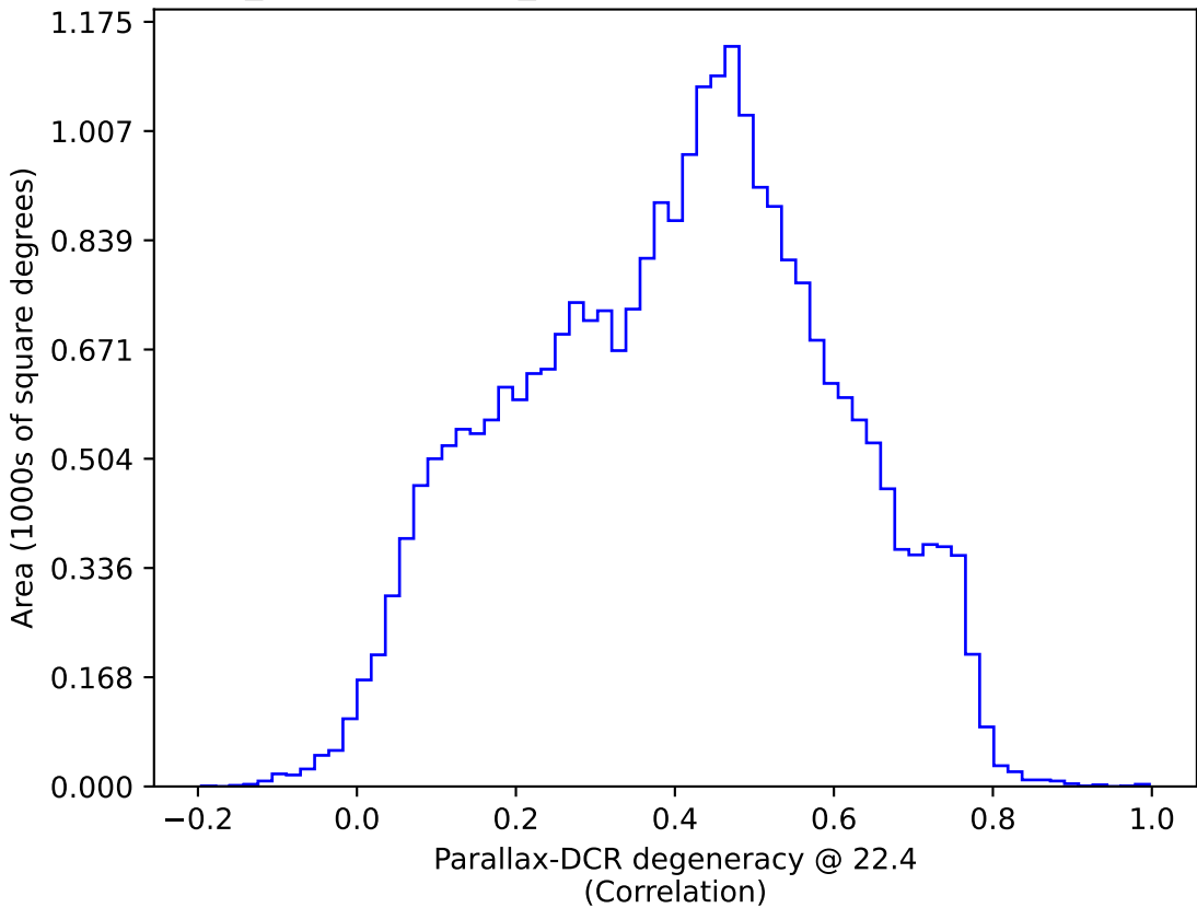
weather_cloudso18v3.4_10yrs : Parallax-DCR degeneracy @ 22.4
