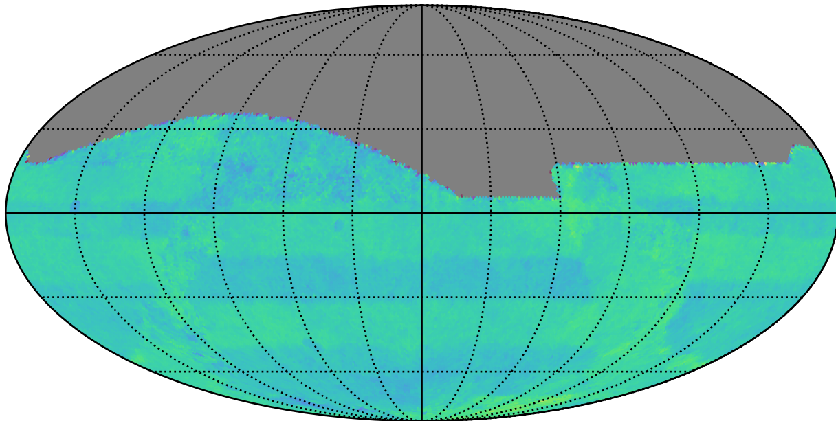
weather_cloudso18v3.4_10yrs : Normalized Proper Motion Uncert @ 24.0
