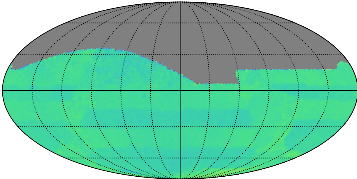
weather_cloudso18v3.4_10yrs : Normalized Proper Motion Uncert @ 20.5
