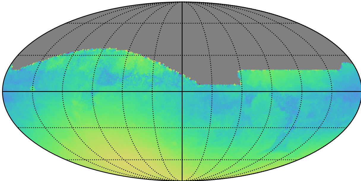
weather_cloudso18v3.4_10yrs : Normalized Parallax Uncert @ 24.0
