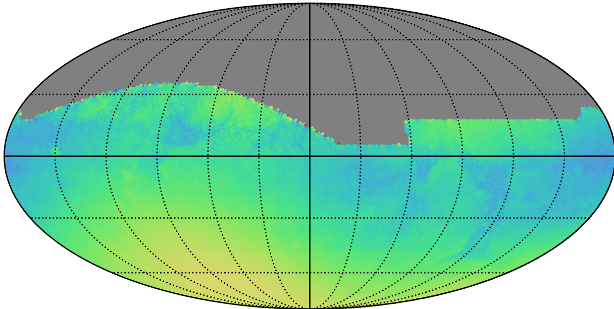
weather_cloudso18v3.4_10yrs : Normalized Parallax Uncert @ 22.4
