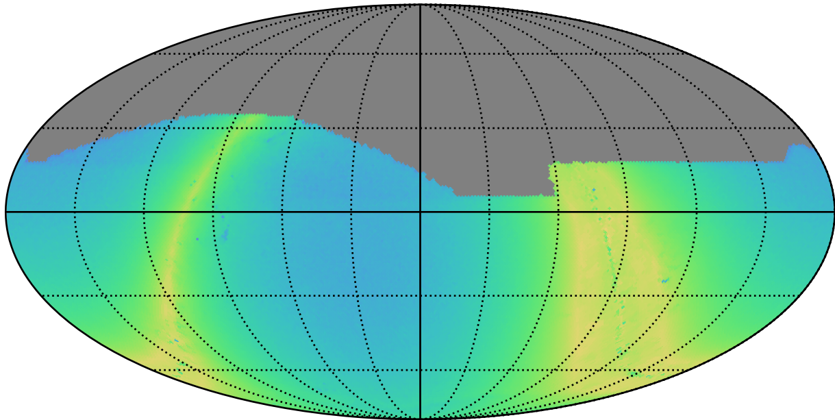
weather_cloudso18v3.4_10yrs z: N stars to Precision 0.20
