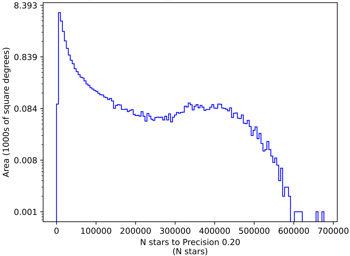
weather_cloudso18v3.4_10yrs z: N stars to Precision 0.20
