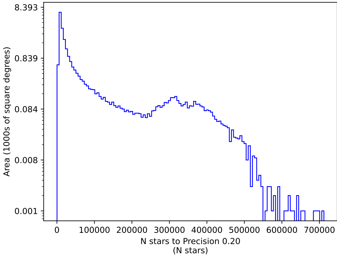
weather_cloudso18v3.4_10yrs y: N stars to Precision 0.20
