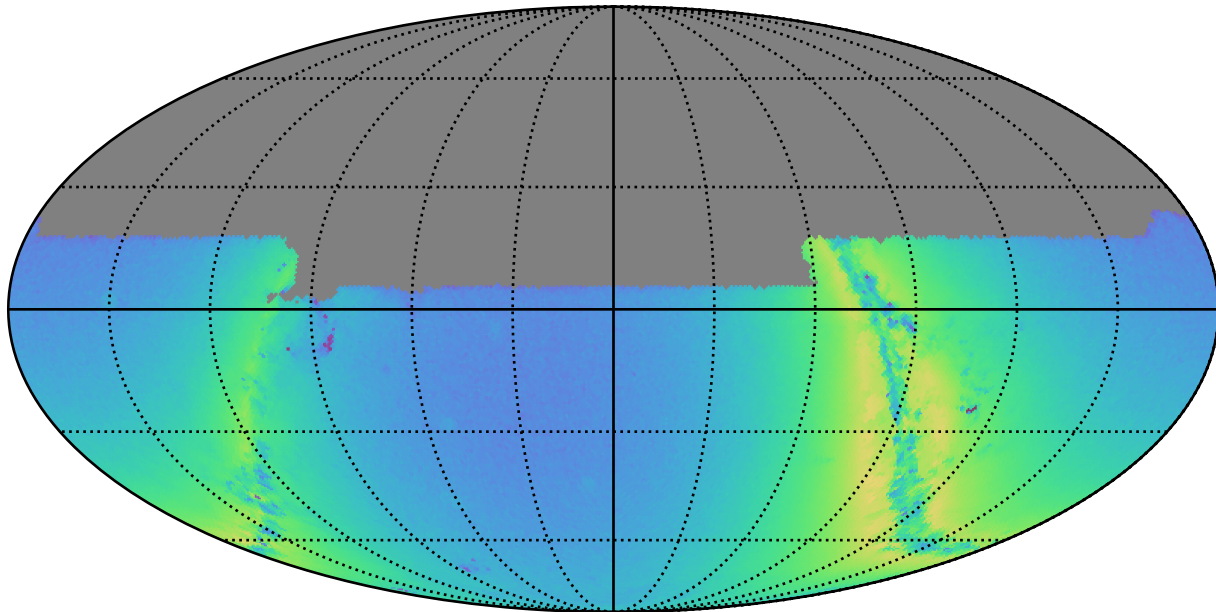
weather_cloudso18v3.4_10yrs u: N stars to Precision 0.20
