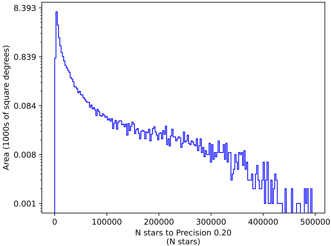
weather_cloudso18v3.4_10yrs u: N stars to Precision 0.20
