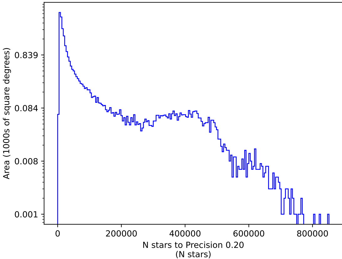
weather_cloudso18v3.4_10yrs r: N stars to Precision 0.20
