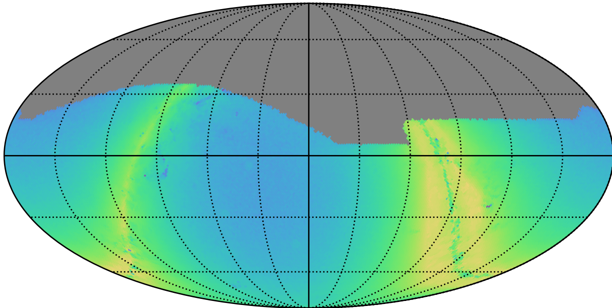
weather_cloudso18v3.4_10yrs g: N stars to Precision 0.20
