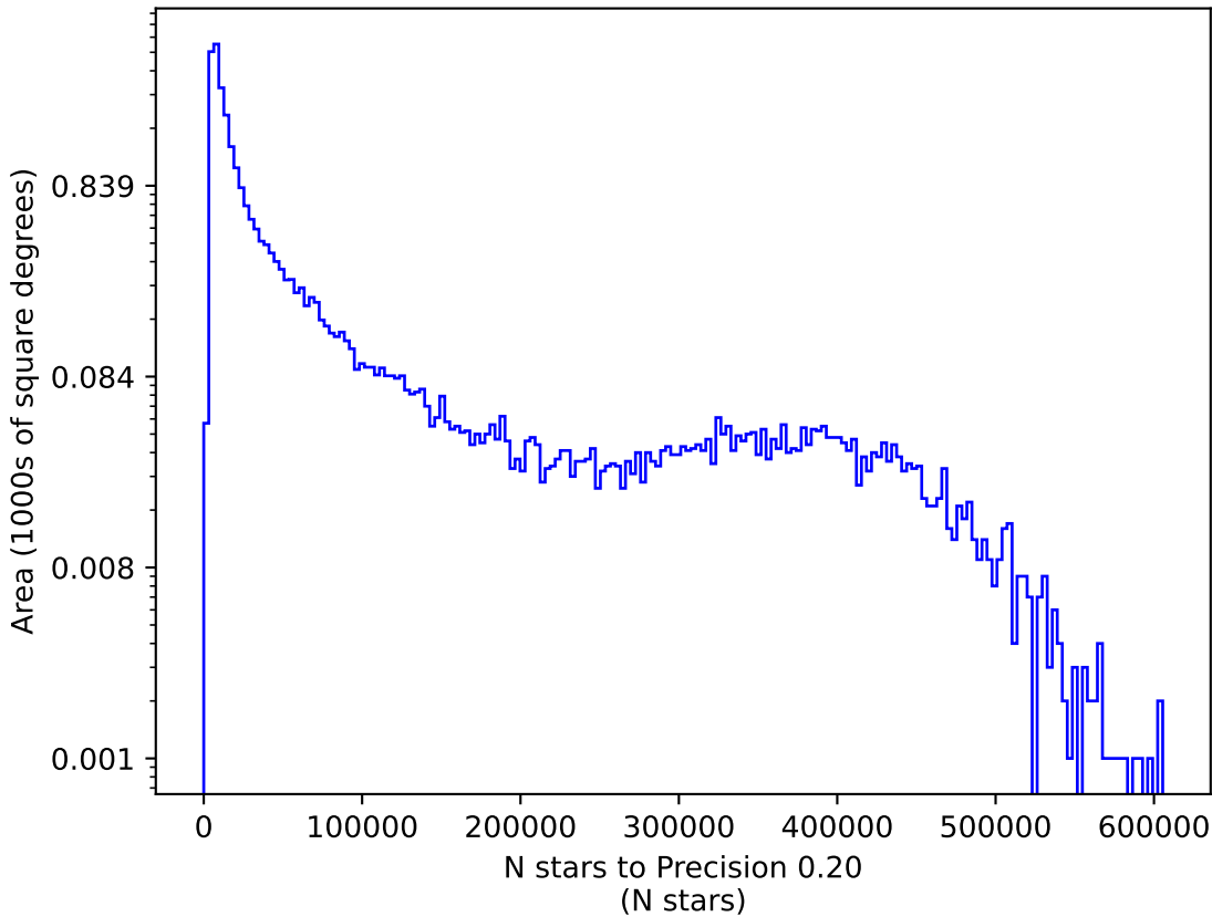
weather_cloudso18v3.4_10yrs g: N stars to Precision 0.20
