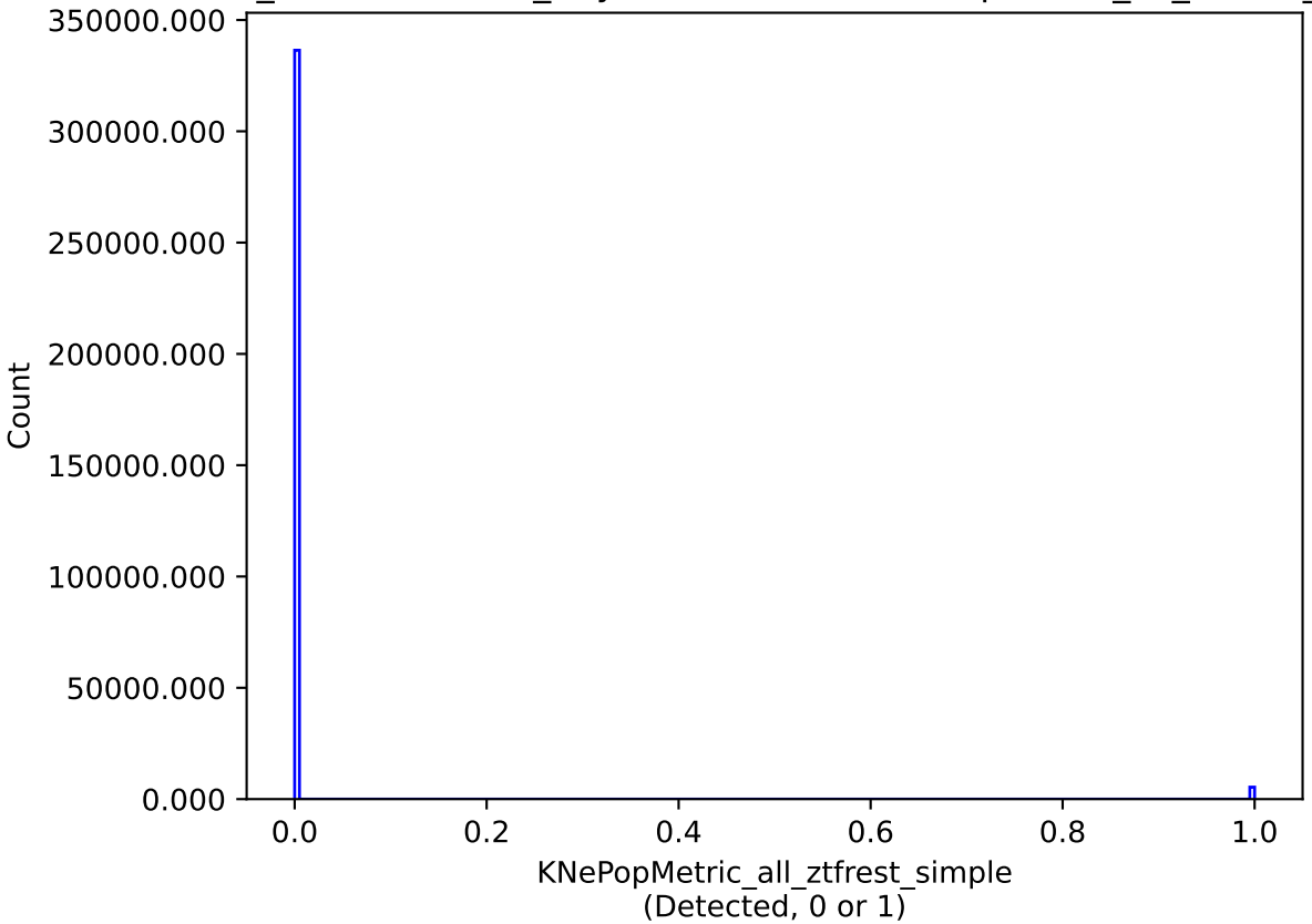
weather_cloudso18v3.4_10yrs all models: KNePopMetric_all_ztfrest_simple
