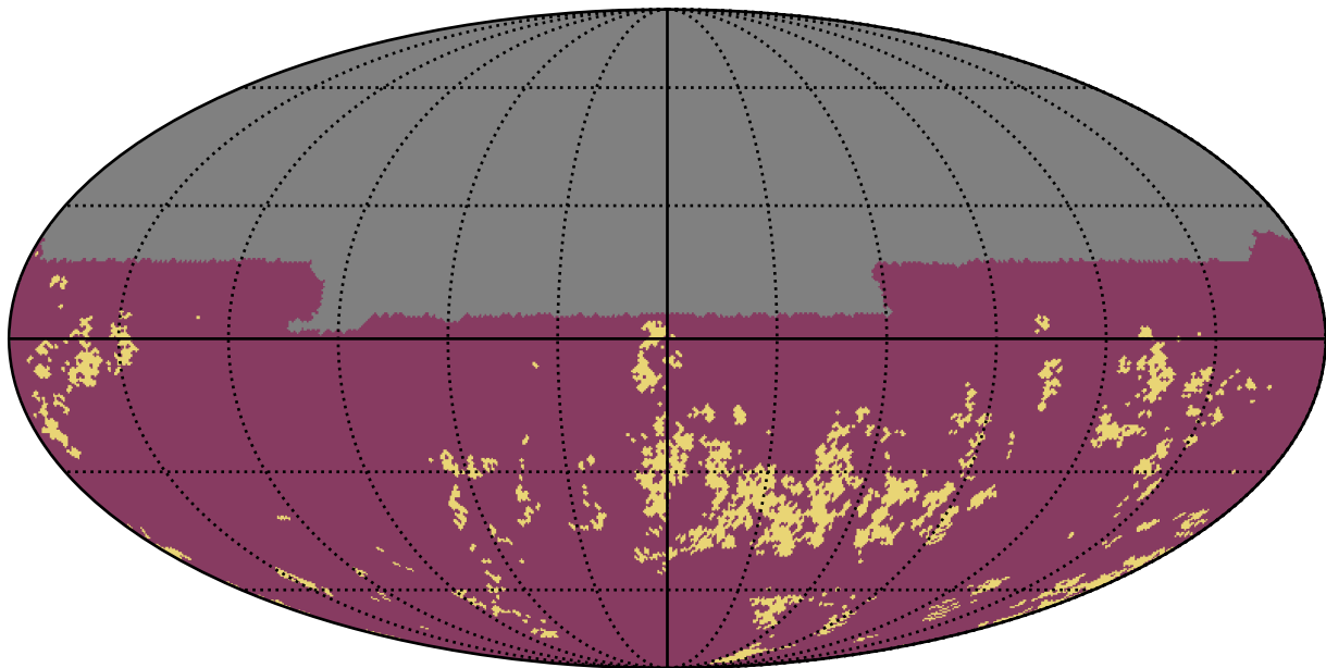
weather_cloudso18v3.4_10yrs u band: Gaps_7hr
