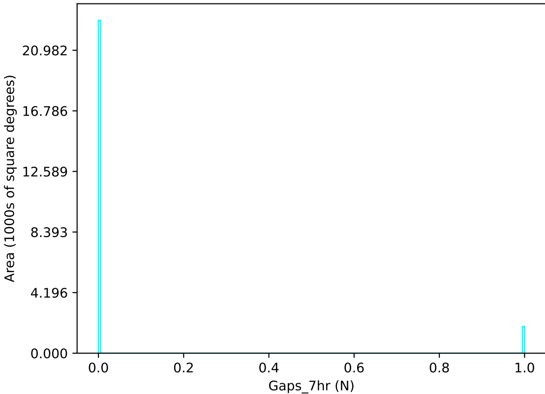
weather_cloudso18v3.4_10yrs u band: Gaps_7hr
