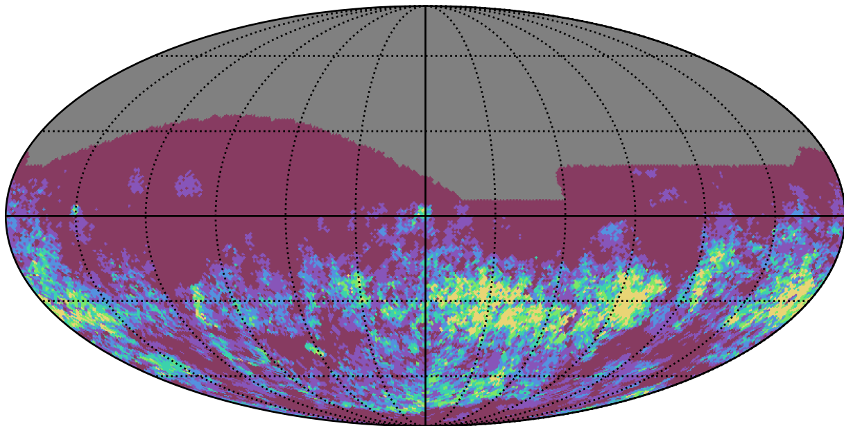
weather_cloudso18v3.4_10yrs r band: Gaps_7hr
