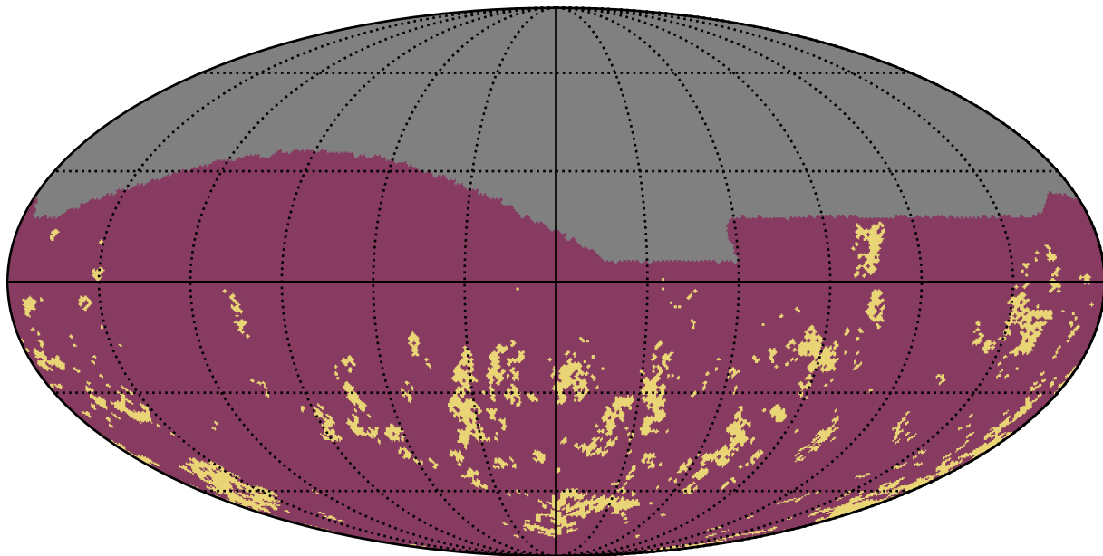
weather_cloudso18v3.4_10yrs g band: Gaps_7hr
