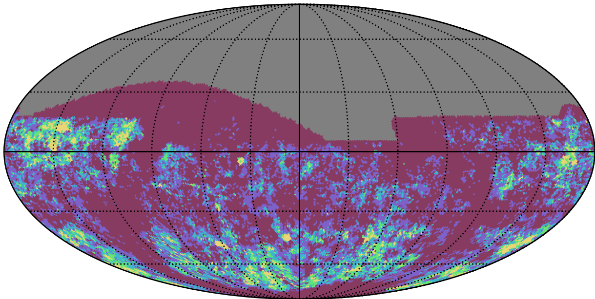
weather_cloudso18v3.4_10yrs z band: Gaps_3hr
