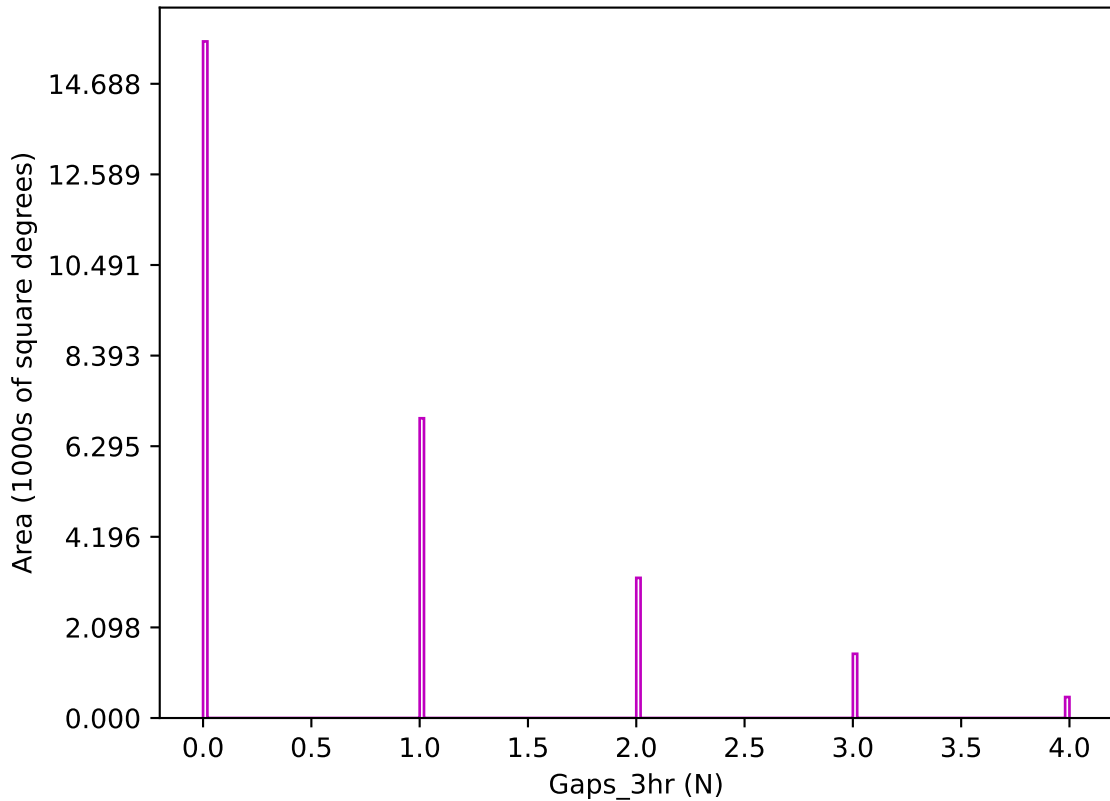
weather_cloudso18v3.4_10yrs z band: Gaps_3hr
