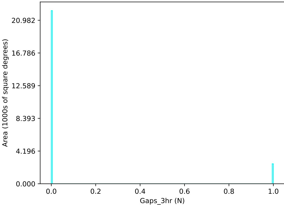
weather_cloudso18v3.4_10yrs u band: Gaps_3hr
