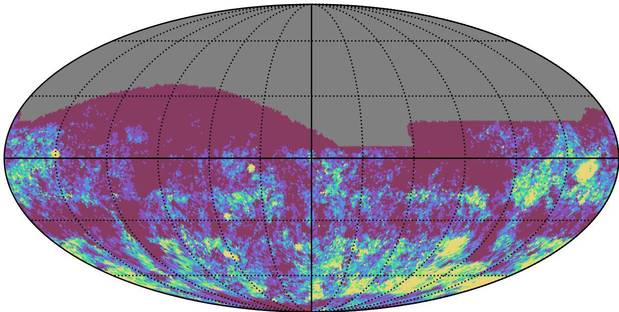
weather_cloudso18v3.4_10yrs r band: Gaps_3hr
